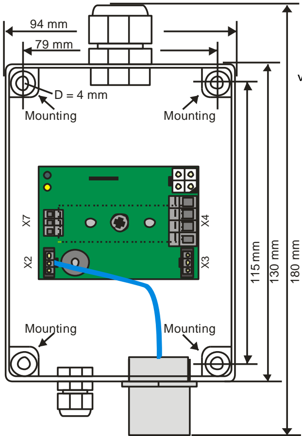
Fig. 1 Basis Sensor Board with Sensor Cartridge
